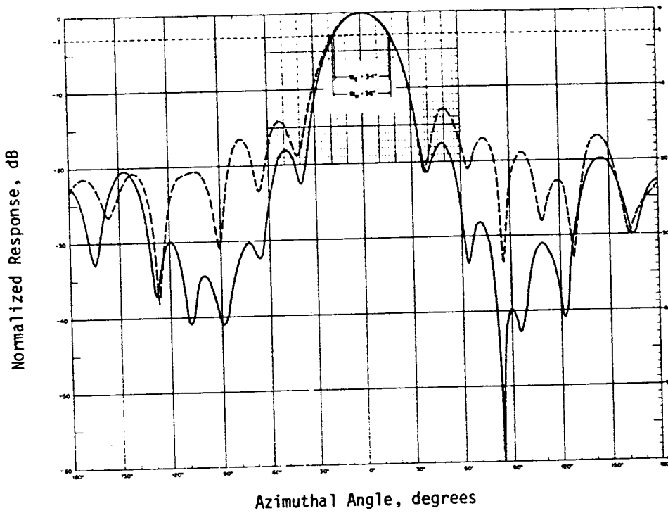
FIG. 17 RADIATION PATTERNS OF A 12-ELEMENT, 2.2\lambda LONG YAGI
