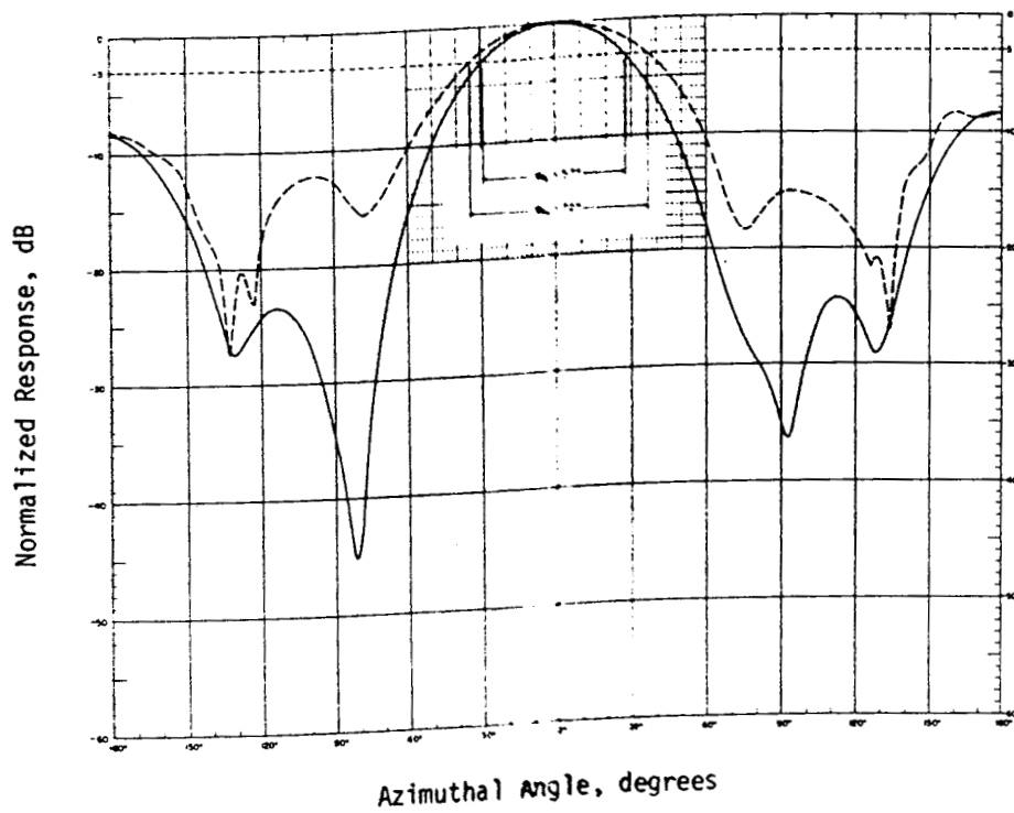
FIG. 14 RADIATION PATTERNS OF A 3-ELEMENT, 0.4\lambda LONG YAGI
