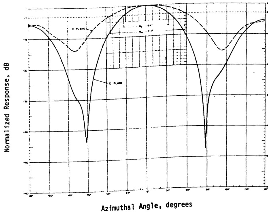
FIG. 13 RADIATION PATTERNS OF A DIPOLE AND REFLECTOR WITH 0.2\lambda SPACING
