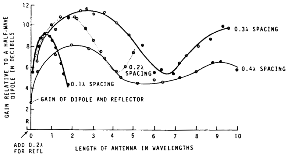
FIG. 5 GAIN OF A YAGI AS A FUNCTION OF LENGTH (NUMBER OF DIRECTORS) FOR DIFFERENT CONSTANT SPACINGS BETWEEN DIRECTORS OF LENGTH EQUAL TO 0.411\lambda
