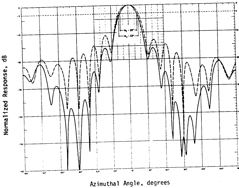
FIG. 18 RADIATION PATTERNS OF A 17-ELEMENT, 3.2\lambda LONG YAGI
