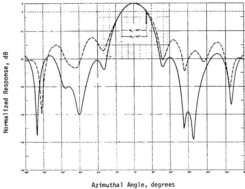
FIG. 16 RADIATION PATTERNS OF A 6-ELEMENT, 1.2\lambda LONG YAGI
