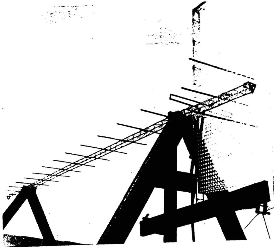
FIG. 3 PHOTOGRAPH OF THE TRIGONAL REFLECTOR EXPERIMENTAL SET-UP USED WITH THE 4.2\lambda YAGI
